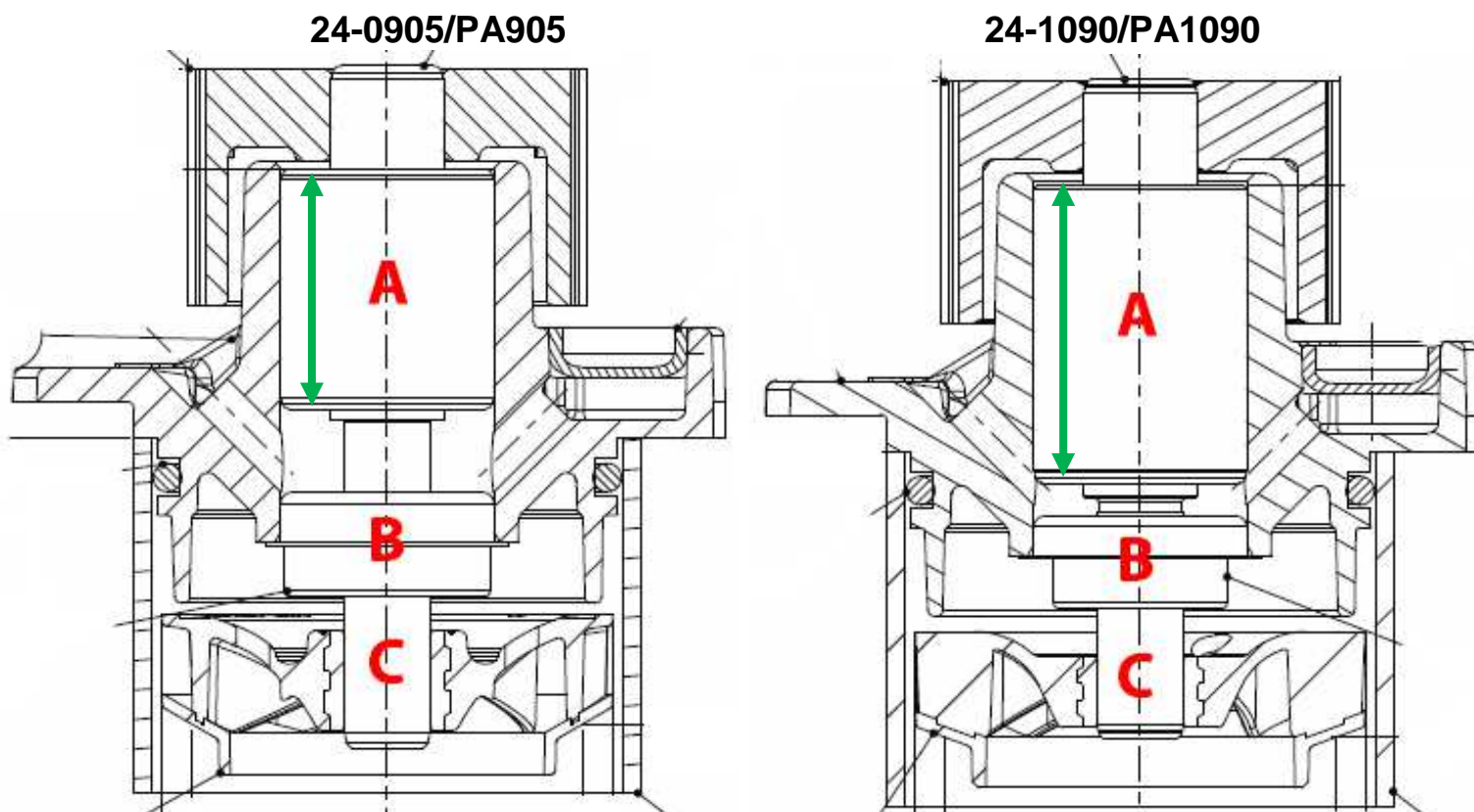
Pic.3: Different parts are equipped on these water pumps
