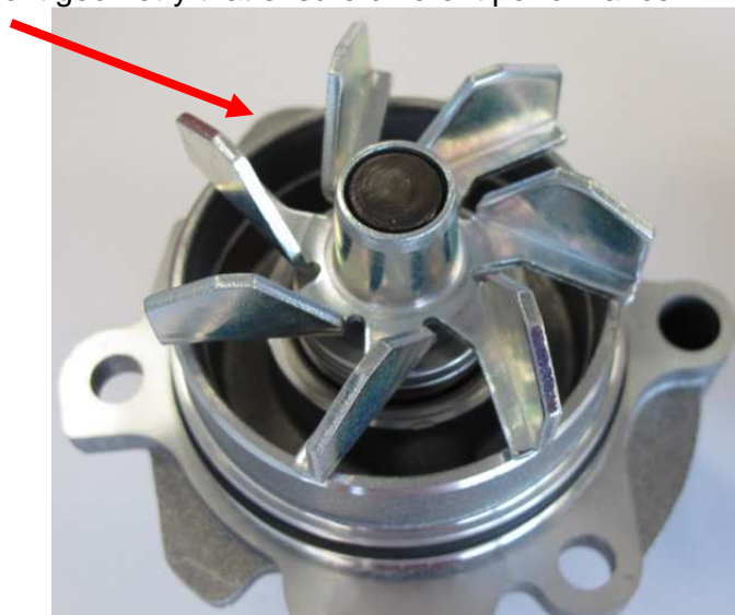
Pic.4: 24-0905/PA905: 7 blades impeller with open shape geometry.
