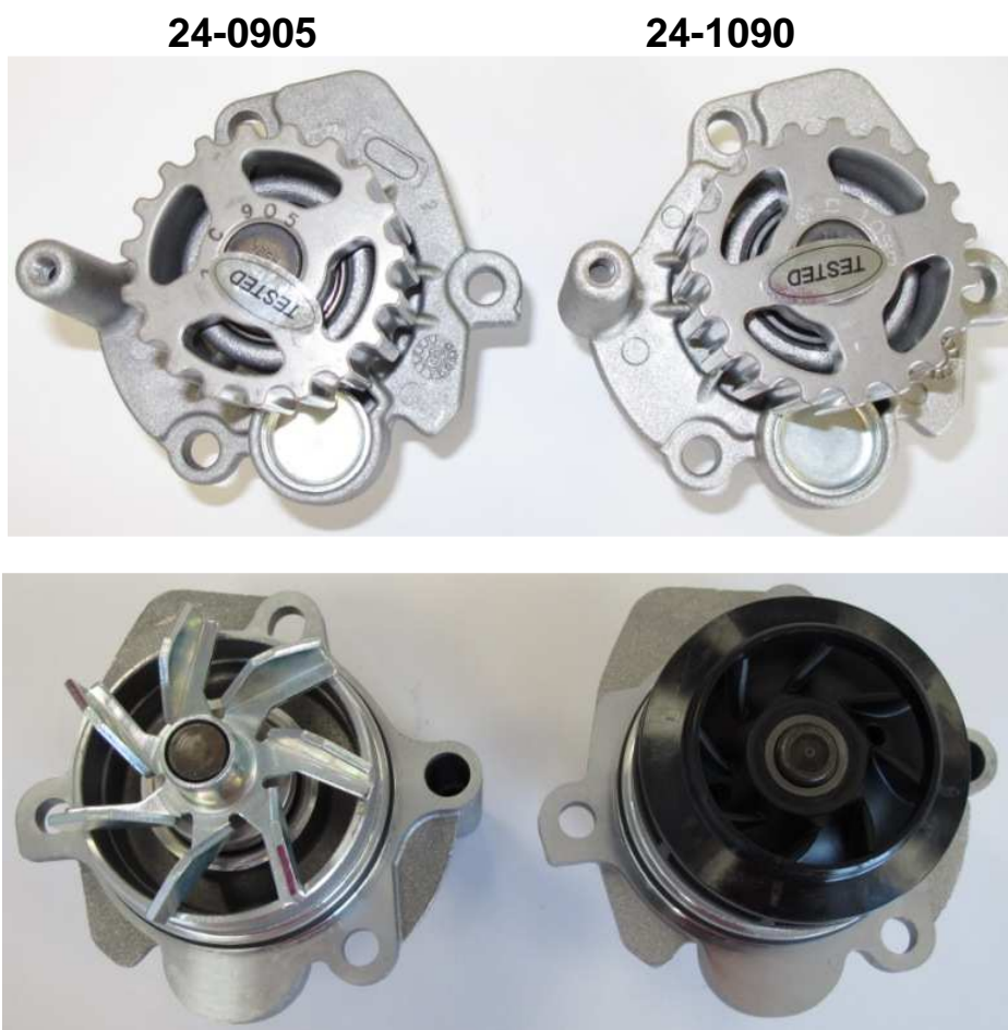
Pic.1: These two water pumps looks like the same product but they hide different technical components that have influence on the performance of the product during the running condition.
